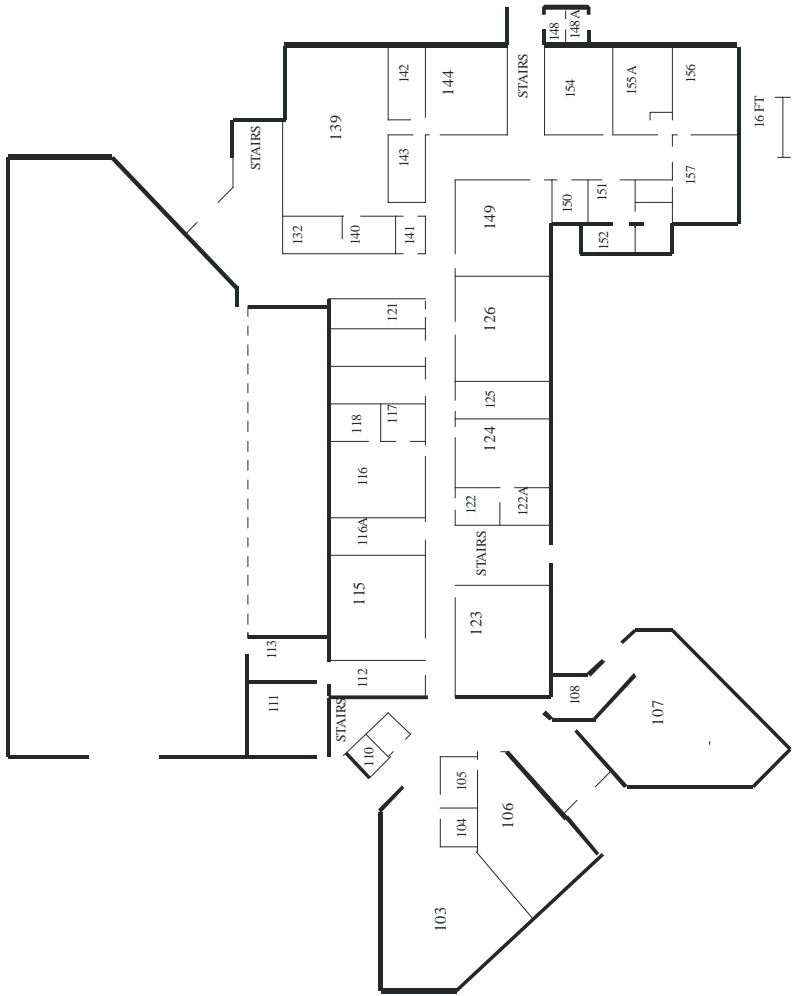
BHNSN 1ST FLOOR SCALE = 1/32" PER FT.
